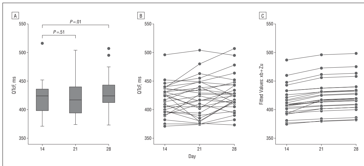
Figure 3. Increase of Fridericia-corrected QT (QTcF) interval value after replacement of ( R )-methadone (day 14) by the initial dose of ( R,S )-methadone (days 21 and 28) (n=29 patients). Box plot (A), individual (B), and multivariate models (C) of QTcF value changes between days 14, 21, and 28. Median and quartiles are shown (bars represent the 95% confidence intervals). xb and Zu represent the linear predictors for the fixed portion and the random portion of the model, respectively.
